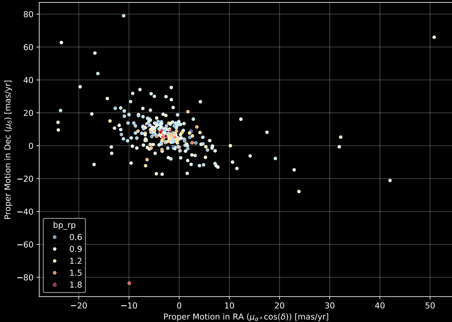
GALAH DR4 Field: [2422] Proper Motion Diagram (n= 254)
