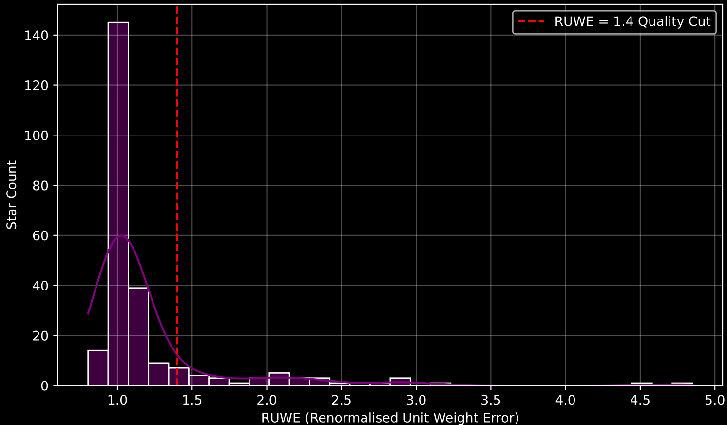
GALAH DR4 Field [2422] RUWE Distribution (n= 244)
