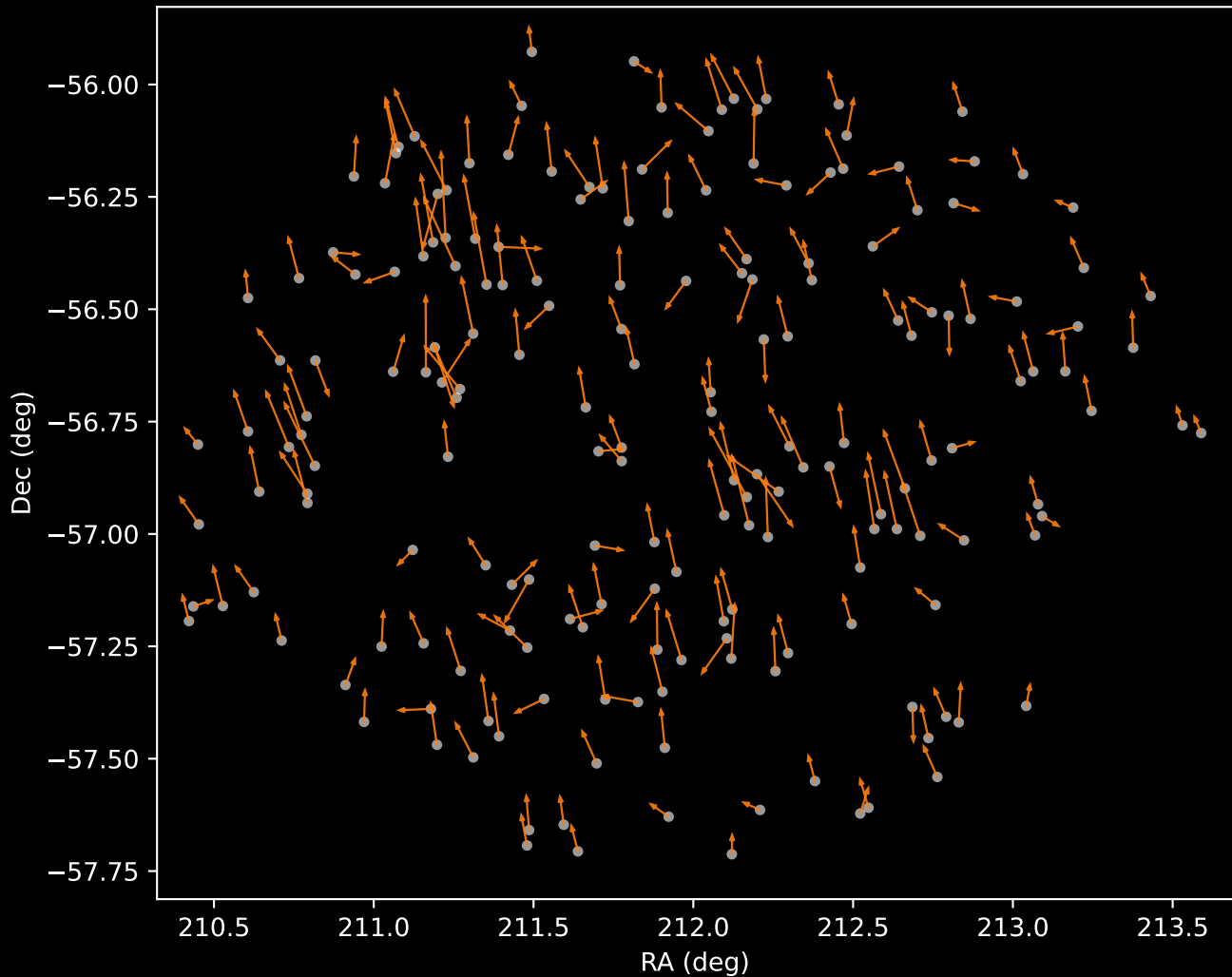
GALAH DR4 Cluster 2 Proper Motion Vectors (n=192)
