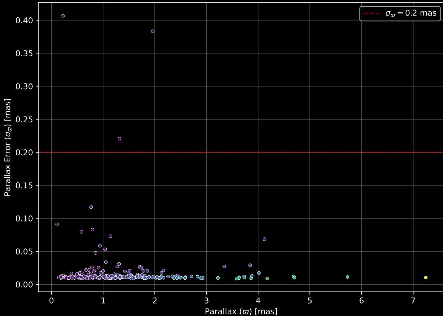
GALAH DR4 Field: [2422] Parallax Quality (n= 254)
