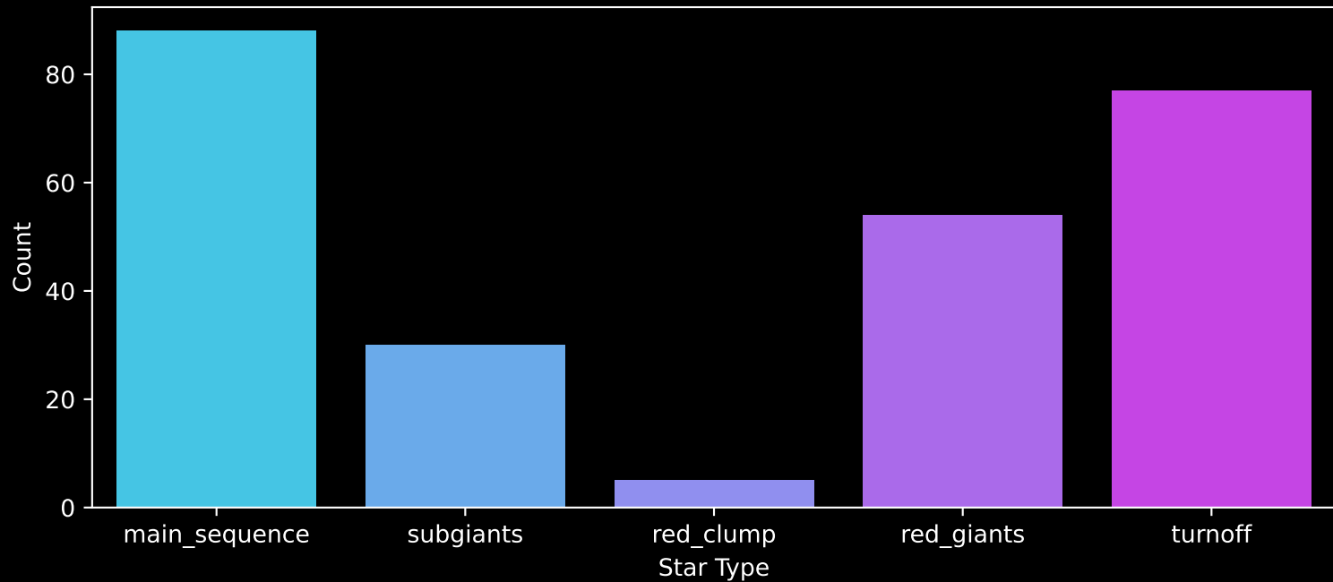
GALAH DR4 Field: [2422] Count plot of Star Type
