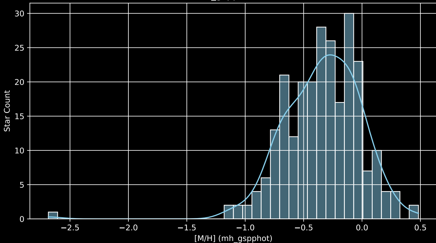
GALAH DR4 Field: [2422] [M/H] (mh_gspphot) (n= 254)
